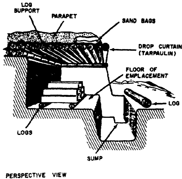
Figure 1-47. Ammunition shelter.
